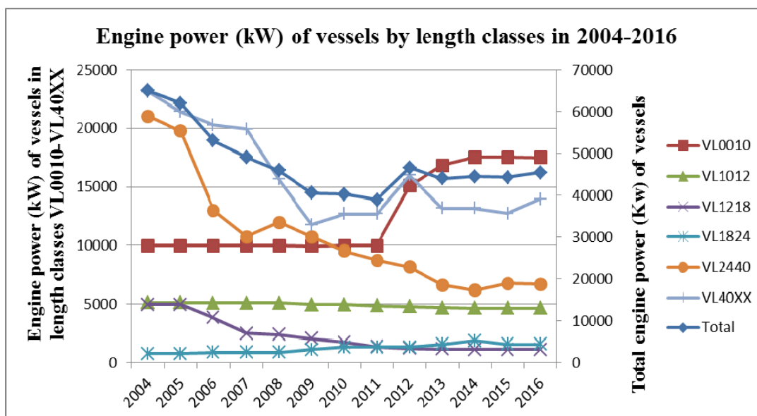
Chart 7. Developments in the main engine power of vessels in Estonian marine fishing fleet by vessel length classes in 2004-2016.
