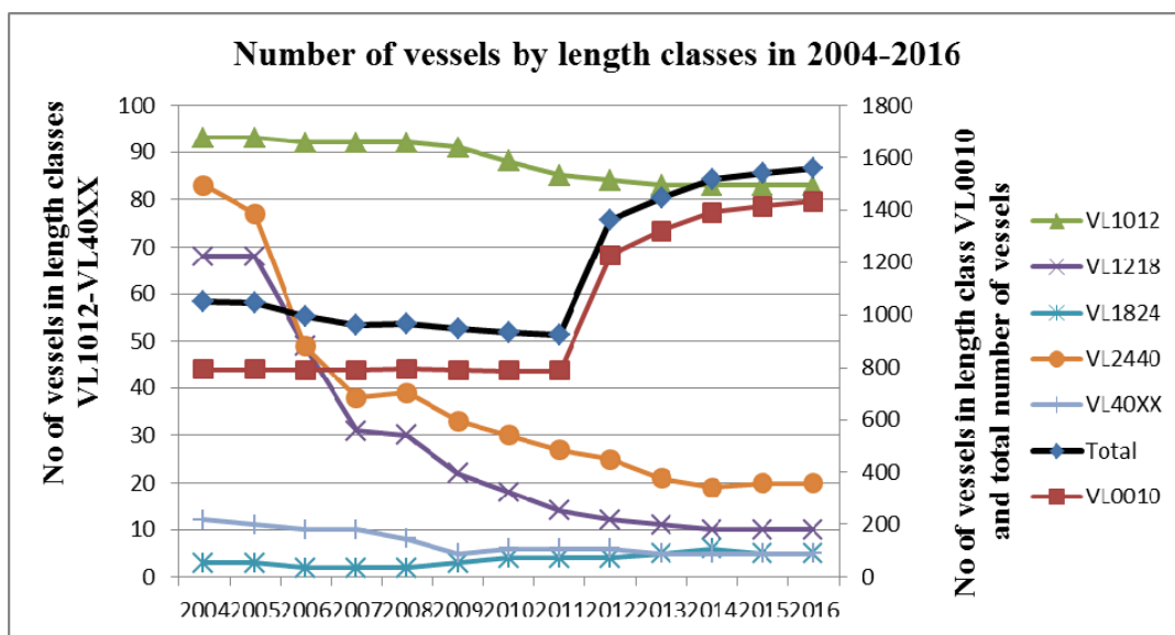
Chart 6. Developments in the number of vessels in Estonian marine fishing fleet by vessel length classes in 2004-2016.
